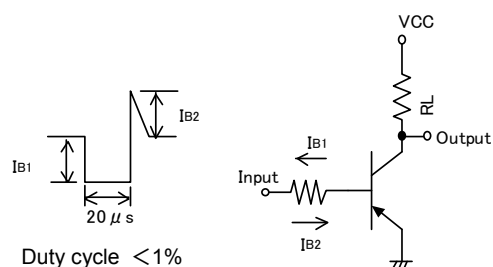
Figure 3. Switching Time Test Circuit & Timing Chart
